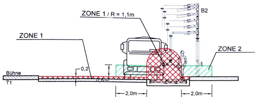
Hazardous areas at bottomloading
