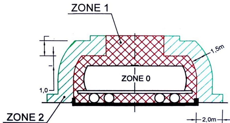
Hazardous area at a road tanker
