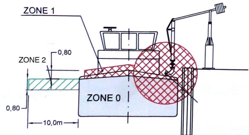
Hazardous areas at a shipping pier
